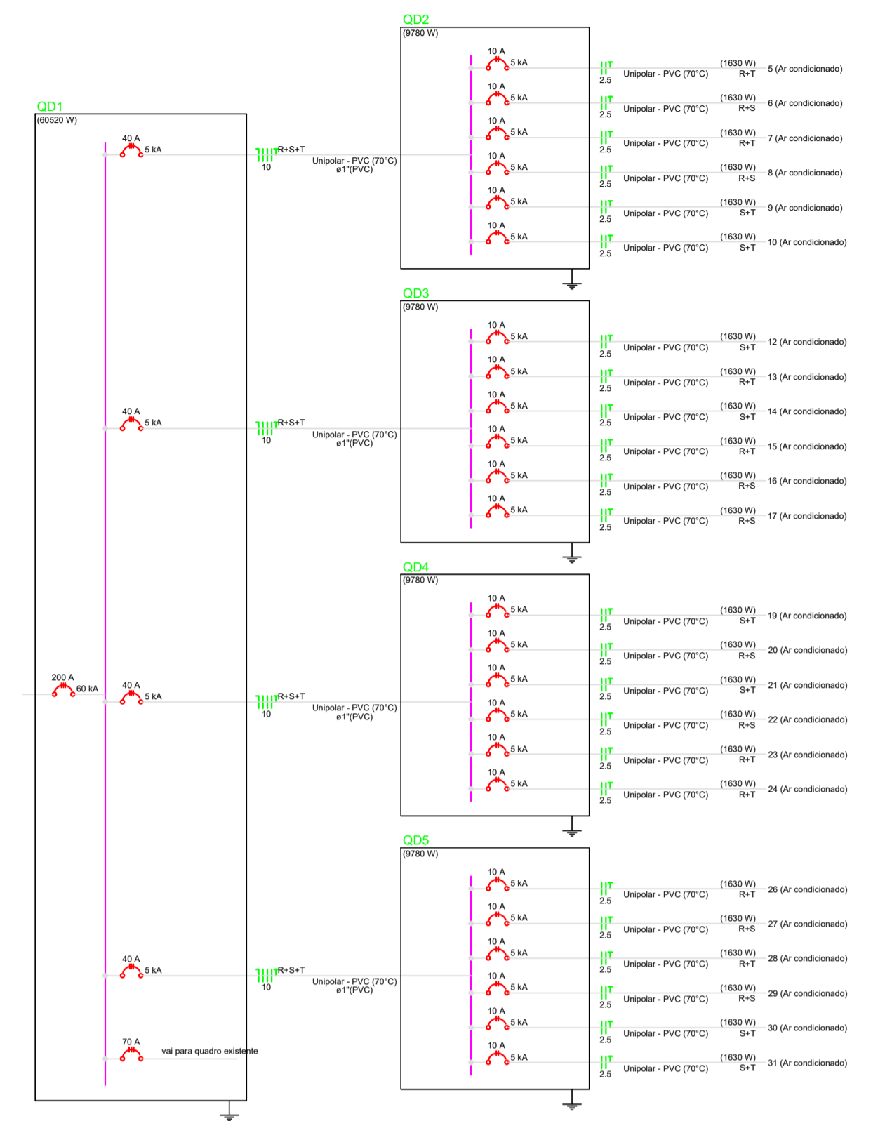
Diagrama Unifilar
